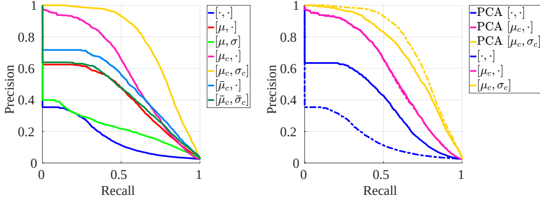
Fig. 4 Comparing MCNCC to baselines for image retrieval within the same domain. The methods are denoted by two operations in square brackets: mean subtraction and normalization, respectively. \mu and \sigma denote computing the statistics across all channels, \mu_c and \sigma_c denote computing per-channel statistics, and \cdot denotes the absence of the operation ( e.g. , MCNCC is denoted as [\mu_c, \sigma_c] , whereas cross-correlation is denoted as [\cdot, \cdot] ). Finally, \bar{\mu}_c and \bar{\sigma}_c denote computing the average per-channel statistics across the dataset. The left panel shows the performance on the raw features, whereas the right panel compares globally whitened features using PCA (solid lines) against their corresponding raw features (dot-dash lines). (Best viewed in color.)
