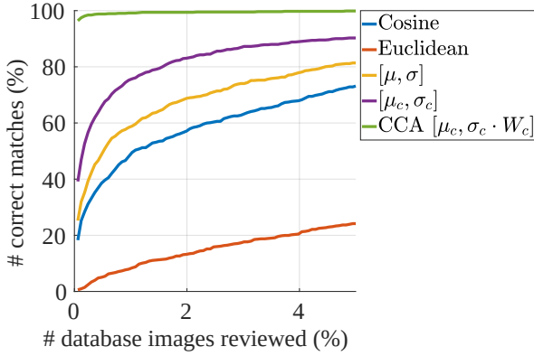
Fig. 7 Segmentation retrieval for building facades. The left panel compares MCNCC with learned linear projections and per-channel importance weights (denoted as CCA [\mu_c, \sigma_c \cdot W_c] ) and MCNCC with no learning (denoted as [\mu_c, \sigma_c] ) to other baseline metrics: Cosine similarity, Euclidean distance, and NCC using across-channel local statistics (denoted as [\mu, \sigma] ). The right panel shows retrieval results for CCA [\mu_c, \sigma_c \cdot W_c] . The left column shows the query facade image. Green boxes indicate the corresponding ground truth segmentation label.
