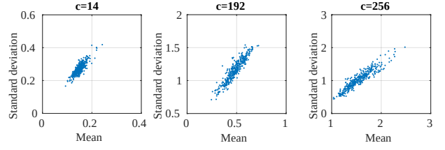
Fig. 3 Normalizing channel statistics: As shown in the histograms of Fig. 2, for some feature channels, patches have wildly different means and standard deviations. For channel 14 (left), the statistics (and hence normalization) are similar from one patch to the next while for channel 256 (right), means and standard deviations vary substantially across patches. CNN channel activations are positive so means and standard deviations are strongly correlated.
