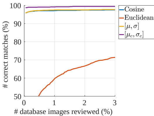
Fig. 8 Retrieval of maps from aerial imagery. The left panel compares MCNCC with no learning (denoted as [\mu_c, \sigma_c] ) to other baseline metrics: Cosine similarity, Euclidean distance, and NCC using across-channel local statistics (denoted as [\mu, \sigma] ). The right panel shows retrieval results for [\mu_c, \sigma_c] . The left column shows the query aerial photo. Green boxes indicate the corresponding ground truth map image.
