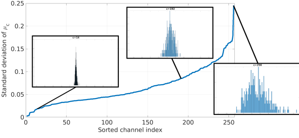
Fig. 2 Distribution of patch channel means: For each query image (patch) we match against the database, our proposed MCNCC similarity measure normalizes ResNet-50 ‘res2x’ feature channels by their individual mean and standard deviation. For uniformly sampled patches, we denote the normalizing mean for channel c using the random variable \mu_c . For each channel, we plot the standard deviation of \mu_c above with channels sorted by increasing standard deviation. When the mean response for a channel varies little from one patch to the next (small std, left), we can expect that a global, per-dataset transformation (e.g., PCA or CCA whitening) is sufficient to normalize the channel response. However, for channels where individual patches in the dataset have very different channel means (large std, right), normalizing by the local (per-patch) statistics provides additional invariance.
