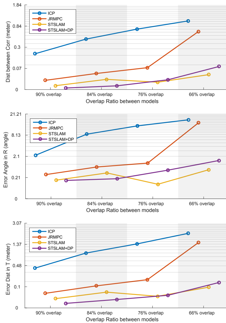
Figure 1. Registration accuracy of our method (STSLAM) compared to (ICP) [1] and joint registration (JRMPC) [2] measured by average closest point distance (Top), rotation angle error (middle), and translation error (bottom).
